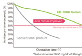
Illuminance maintenance ratio of EB-700U Series*
