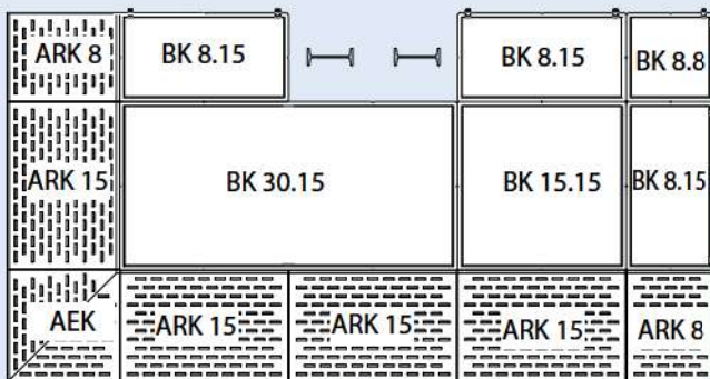
The various dimensions of the floor elements allow you to lay them around posts and supports for example
