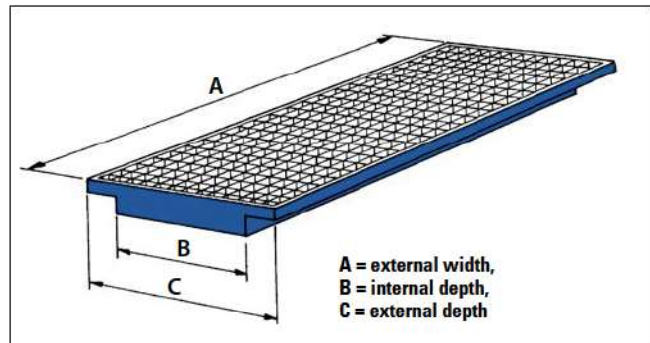
Steel pallet racking sump SRW
