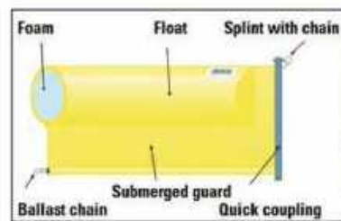
Construction principle for a DENIOS oil barrier
