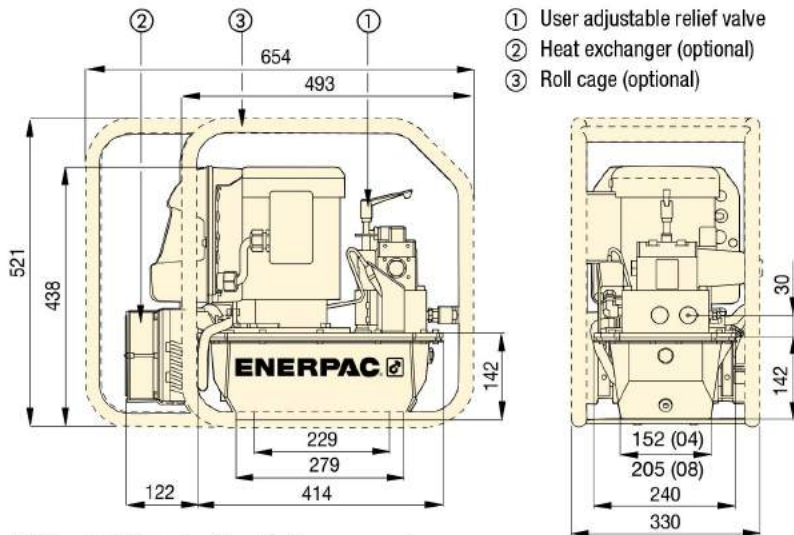
ZE4T and ZE5T-Series, 4 and 8 litres reservoirs
