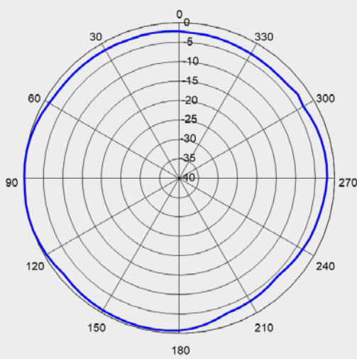
2.4G (PHI=0)
