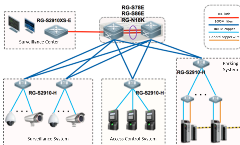
Figure 4: RG-S2910-H Deployment for Smart Building
