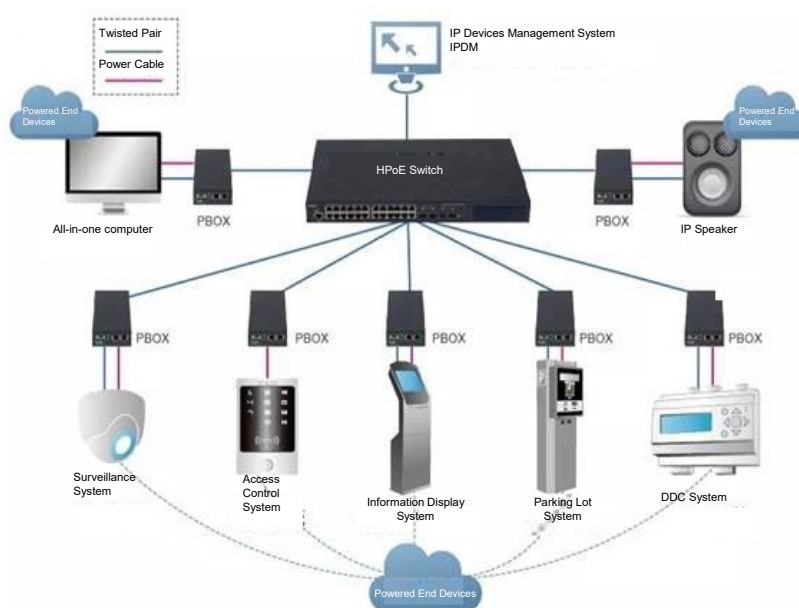
Figure 5: RG-S2910-H Powering the End Devices
