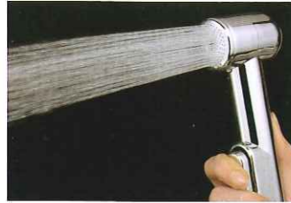
SR- 9201 MATERIAL:ABS WEIGHT:73G WORKING PRESSURE:0.1MPA~1.0MPA
