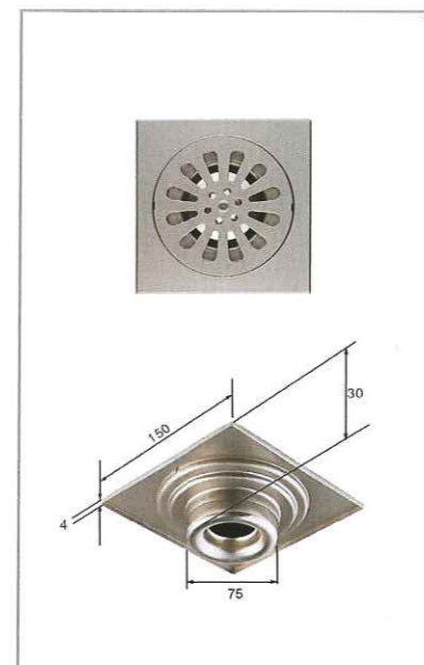
SR- 106 FLOOR DRAIN 150mmx150mm
