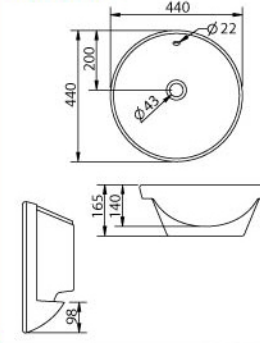
WB2034 Lotite Basin
