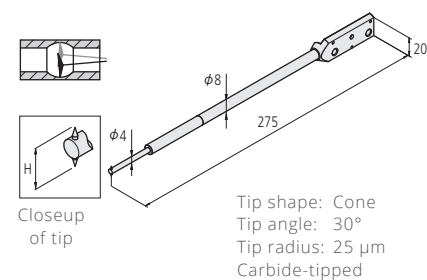
| Double-sided small hole arm stylus SPHW-33
