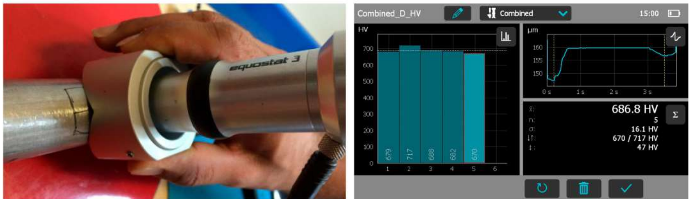
Figure 28: Performing Portable Rockwell measurements and Equotip 550 screen after five measurements
