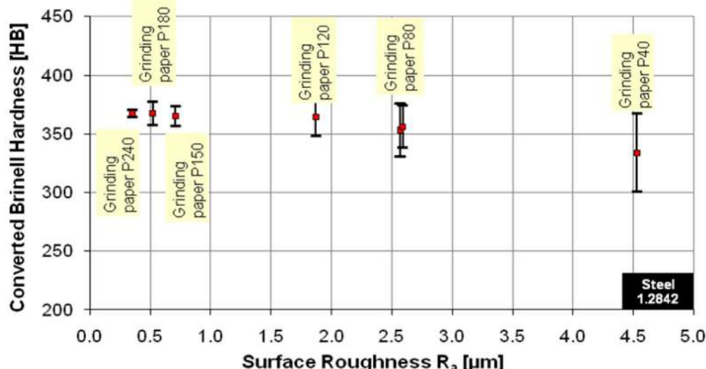
Figure 2: Brinell hardness vs. surface roughness obtained using an Equotip Leeb Impact Device D
