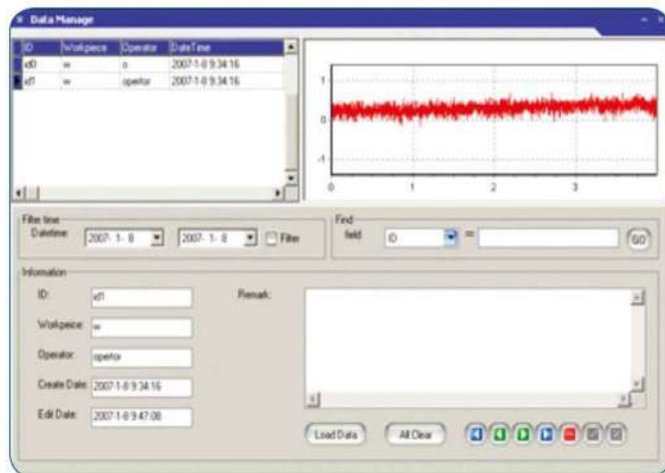
Database management
