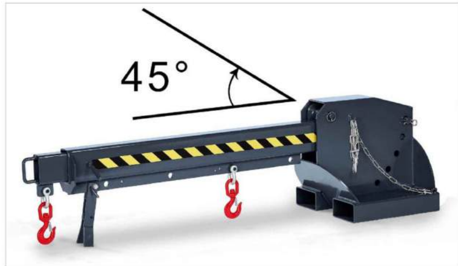
Crane arm, extendable and height-adjustable version (6 extension positions, 5 height adjustments up to 45°)
