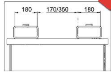
Forklift pockets dimensions (mm), 350 mm for 1000 litres
